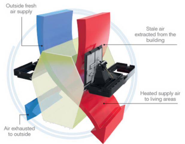
Recovery Mode (Winter Operation Shown)
