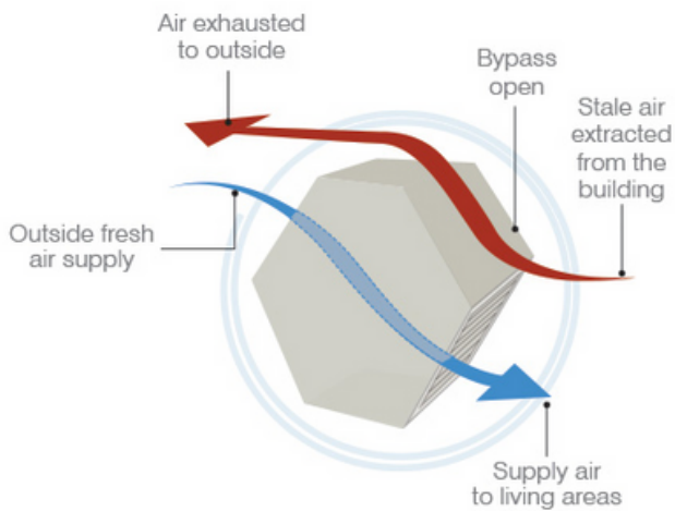
Summer Bypass Mode
